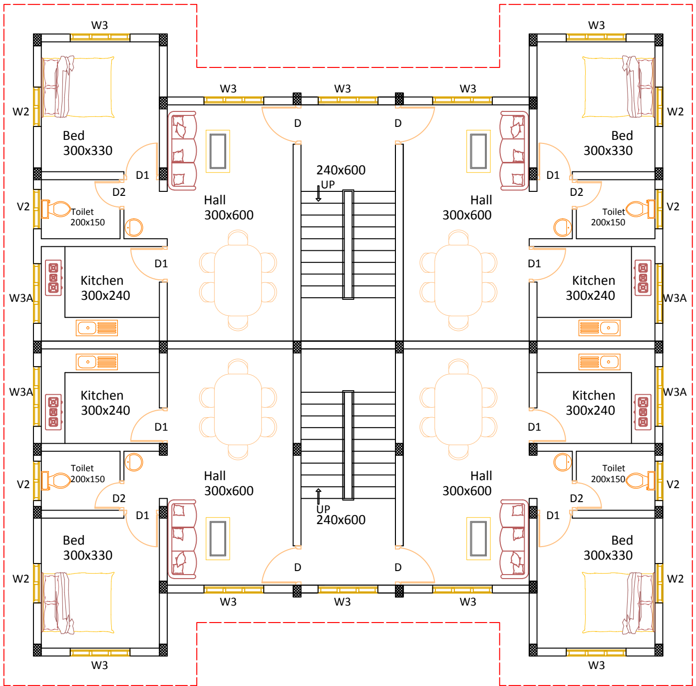
FIRST & SECOND FLOOR PLAN
