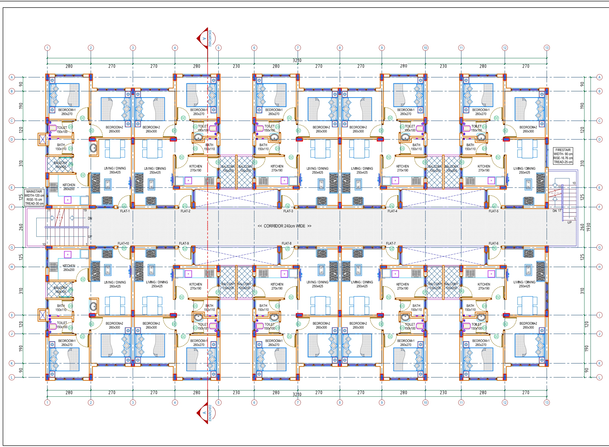
TYPICAL FLOOR PLAN (1ST to 3rd)
